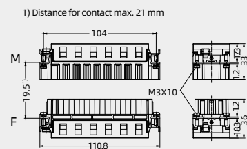
Contact arrangement view from termination side
